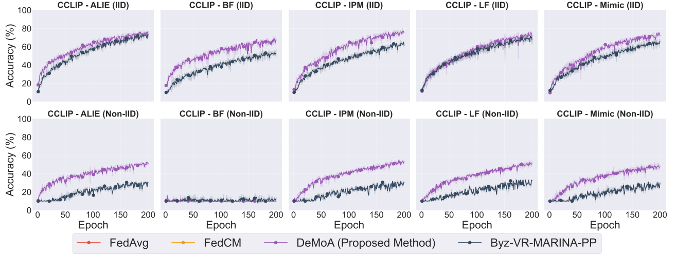
Figure 3. Training with Byzantine ratio \delta = 0.2 using centered clipping (cp) aggregator. The top row shows IID splits and the bottom row shows non-IID splits with bucketing size s = 2 ; from left to right, the columns correspond to ALIE, Bit-Flipping (BF), IPM, Label-Flipping (LF), and Mimic attacks.
